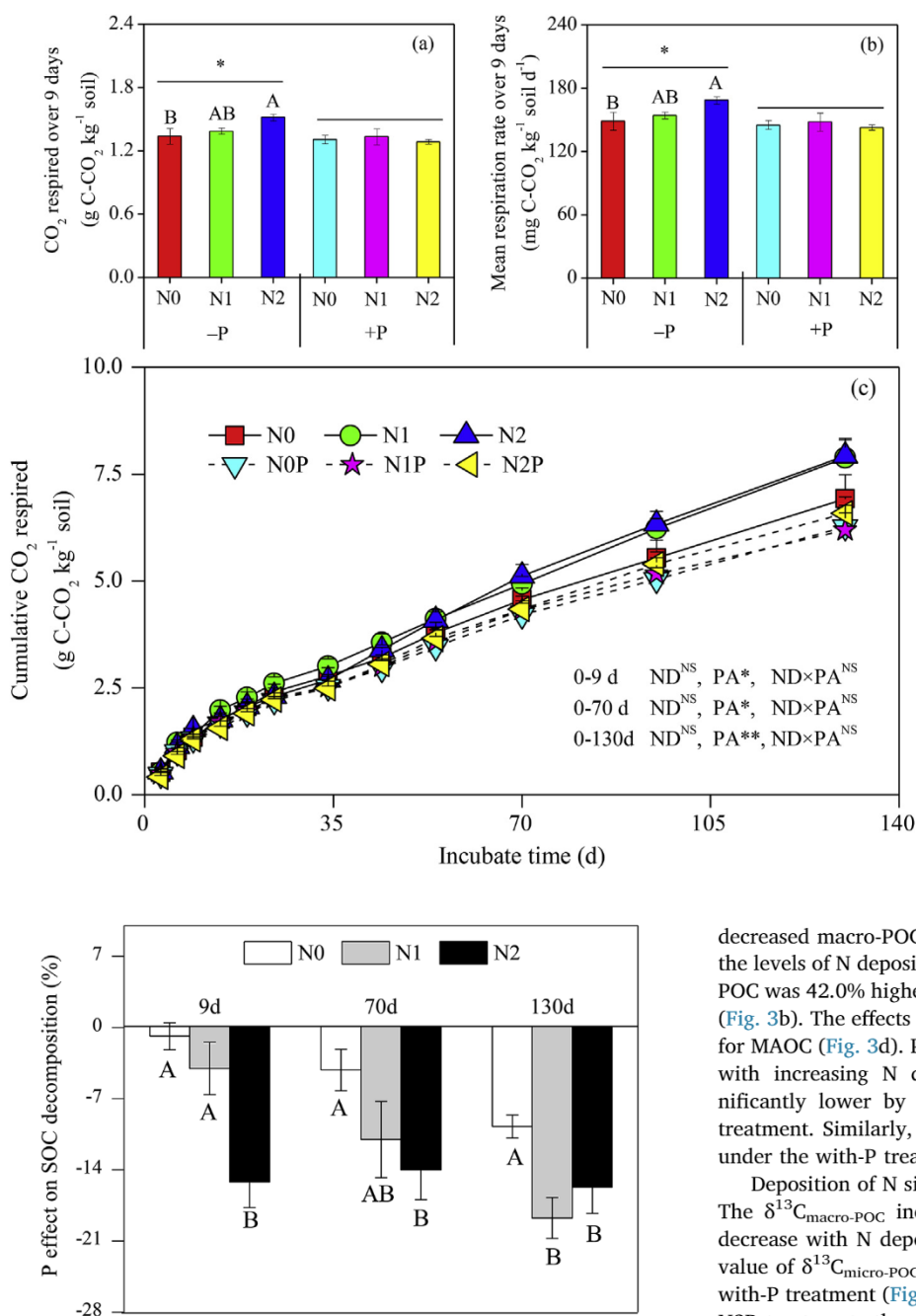
Fig. 2. Response of the P addition effect on SOC decomposition to three N deposition levels. The capital letters indicate the differences among the three levels of N deposition ( p < 0.05 ).
