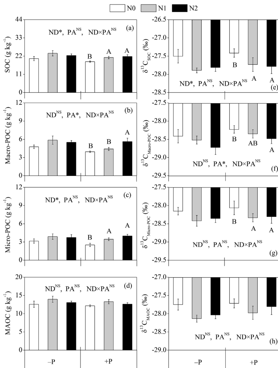
Fig. 3. Effects of N deposition and P additions on SOC (a), particle-size fractions (b–d) and \delta^{13}\text{C} in bulk soil (e) and soil particle samples (f–h) in a subtropical forest. Error bars indicate standard error. ND: nitrogen deposition; PA: phosphorus addition; macro-POC: macro-particulate organic C; micro-POC: micro-particulate organic C; MAOC: mineral-associated organic C; The capital letters indicate the differences among the three levels of N deposition ( p < 0.05 ) in the with-P or without-P treatment. * p < 0.05 ; NS not significant.
