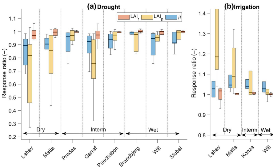
FIGURE 9 Boxplots of the response ratios of the change of \beta , LAI_p and LAI_r , as simulated by (T&C, JSBACH, DLEM, CABLE, JULES and TECO) for the drought experiments (a) and the irrigation experiments (b) [Colour figure can be viewed at wileyonlinelibrary.com ]
