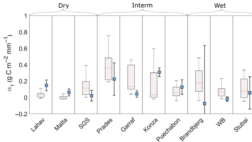
FIGURE 2 Simulated and observed sensitivity of annual aboveground net primary production (ANPP) to annual precipitation ( \alpha_1 = \partial \text{ANPP} / \partial P ). For each site, boxplots indicate the distribution of the simulated sensitivity of ANPP to precipitation by all models. Error bars show the sensitivity of observed ANPP to precipitation (blue squares) and the corresponding 90% confidence intervals (bar length) of the fit of the linear model. Crosses indicate the sites for which the mean value of the distribution of simulated sensitivities is not statistically different from the observed with 90% confidence. Sites are ranked from left to right in order of ascending wetness [Colour figure can be viewed at wileyonlinelibrary.com ]
